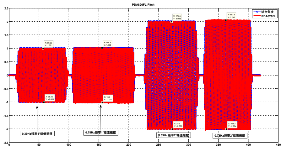
Figure 2. Pitch directional swing data, including 0.39Hz frequency 1 ° amplitude swing, 0.78Hz frequency 1 ° amplitude swing, 0.39Hz frequency 2 ° amplitude swing, and 0.78Hz frequency 2 ° amplitude swing.
