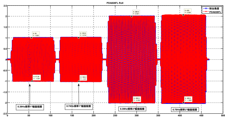
Figure 1. Roll direction swing data, including 0.39Hz frequency 1 ° amplitude swing, 0.78Hz frequency 1 ° amplitude swing, 0.39Hz frequency 2 ° amplitude swing, and 0.78Hz frequency 2 ° amplitude swing.
