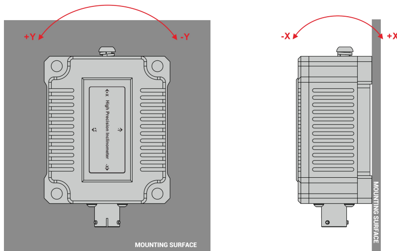
Vertical installation
