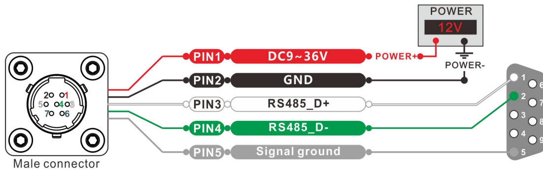
RS422 wiring definition (9-core wiring definition)
